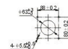
H型手柄面板开孔尺寸
